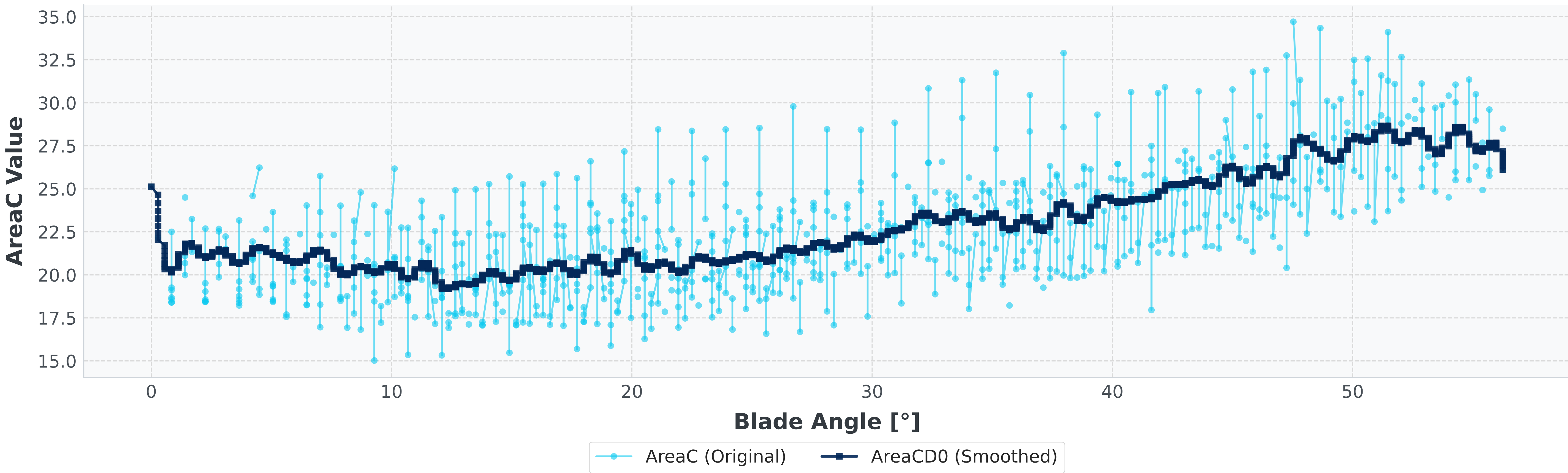
Cavity - AreaC (BLD Phase Averaged)
